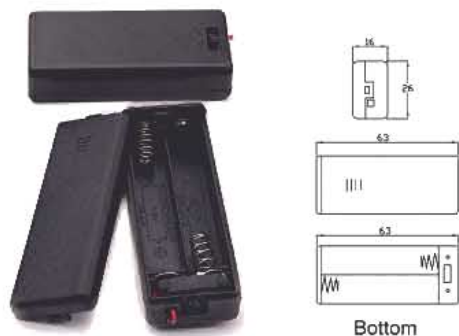
SBH-421-1A SBH-421-1AS FOR TWO "AAA" CELLS
