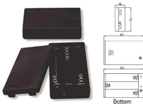
SBH-431-1A SBH-431-1AS FOR THREE "AAA" CELLS
