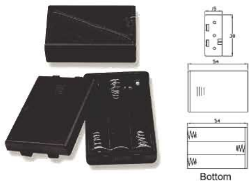
SBH-431A SBH-431B SBH-431D SBH-431P FOR THREE "AAA" CELLS
