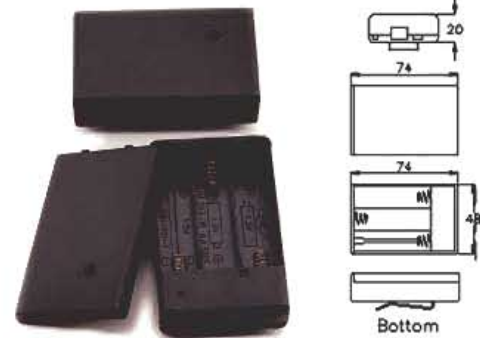
SBH-331-2A SBH-331-2AS FOR THREE "AA" CELLS
