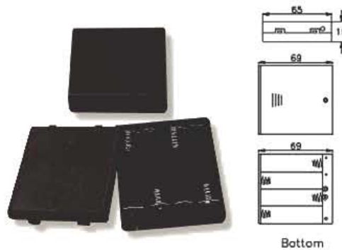
SBH-341A SBH-341AS FOR FOUR "AA" CELLS
