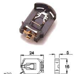
CH7410-2032 FOR CR2032
