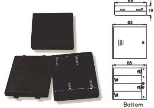
SBH-341-1A SBH-341-1AS FOR FOUR "AA" CELLS
