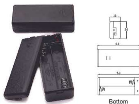
SBH-421-2A FOR TWO "AAA" CELLS
