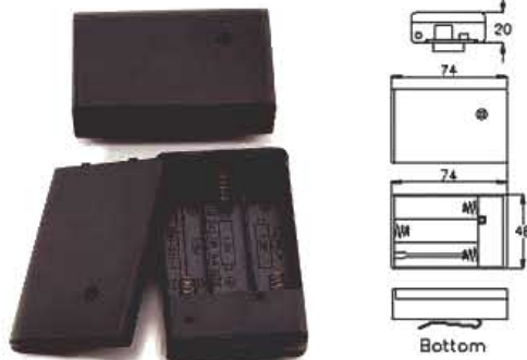
SBH-331-1A SBH-331-1AS FOR THREE "AA" CELLS
