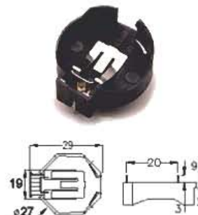
CH273-2450 FOR CR2450
