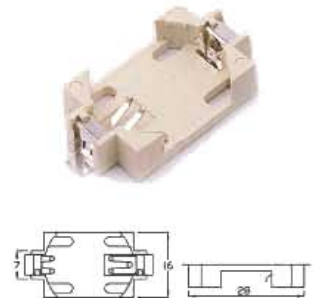
CH28-2032 FOR CR2032
