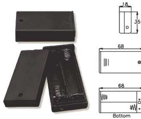
SBH-321-2A FOR TWO 'AA' CELLS
