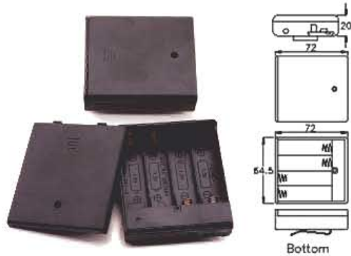
SBH-341-2A SBH-341-2AS FOR FOUR "AA" CELLS
