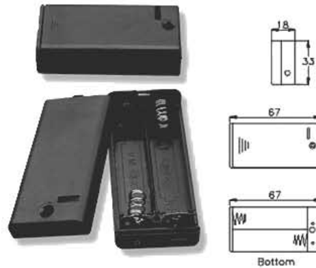
SBH-321A FOR TWO 'AA' CELLS
